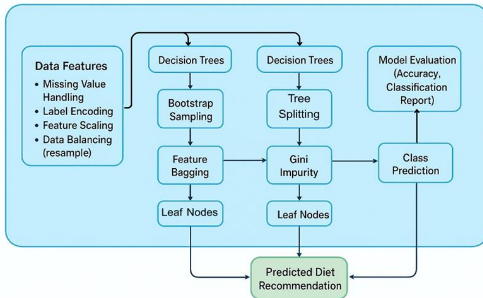
Figure 2: Architecture diagram of diet prediction
