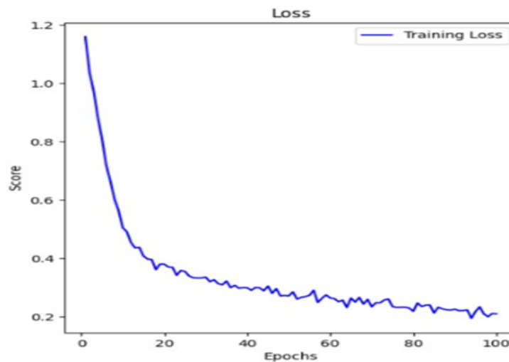
Figure 3: Training loss for 100 epochs
