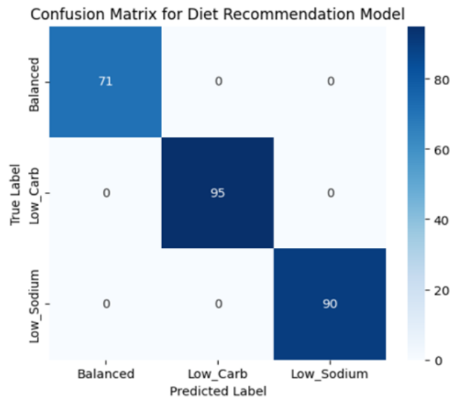
Figure 6: Confusion matrix of diet prediction
