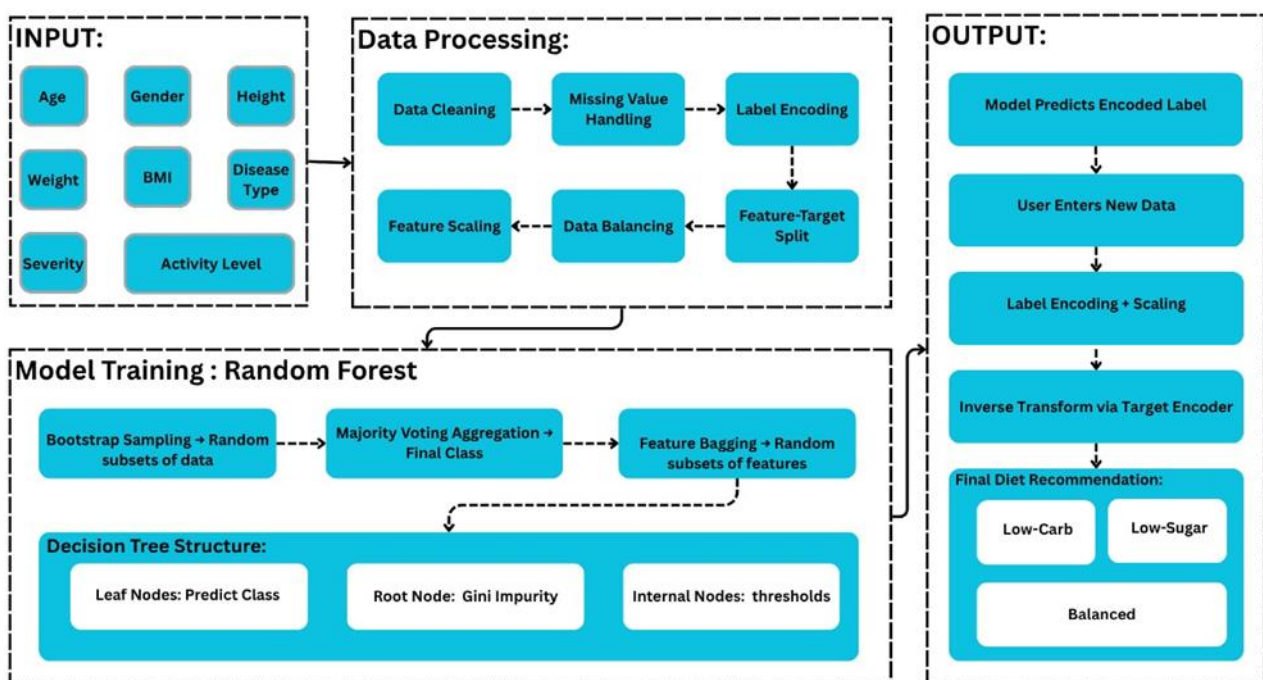
Figure 1: Block diagram of diet prediction
